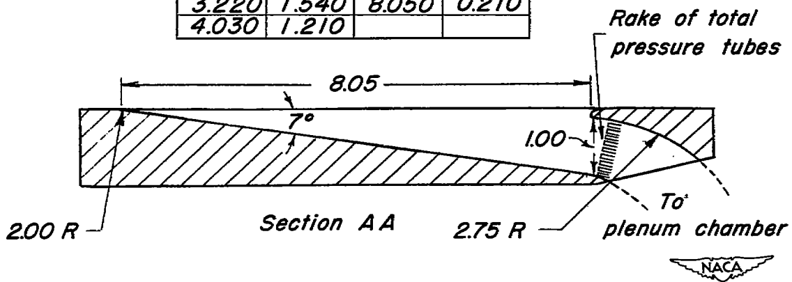
Figure 2.- Drawing of submerged inlet.
